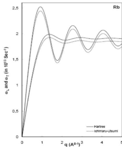
Fig. 4. Phonon dispersion curves of liquid Rb.
