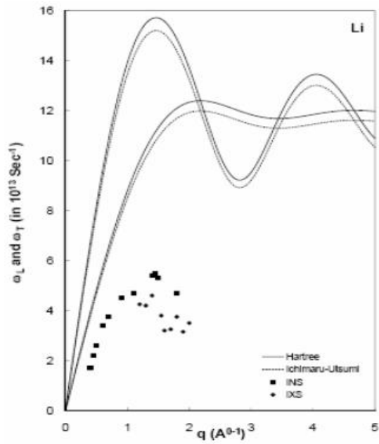
Fig. 1. Phonon dispersion curves of liquid Li.
