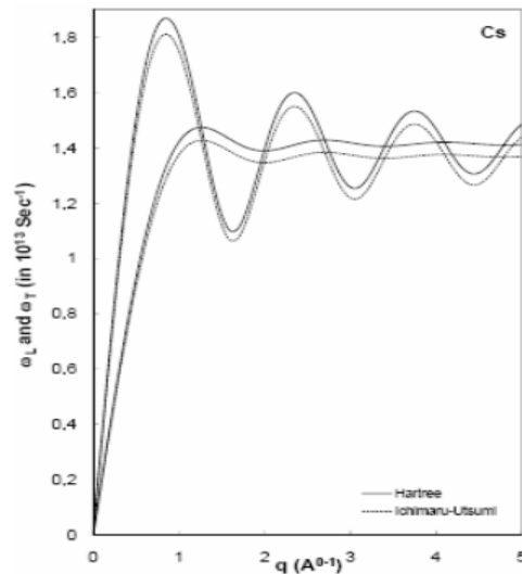
Fig. 5. Phonon dispersion curves of liquid Cs.
