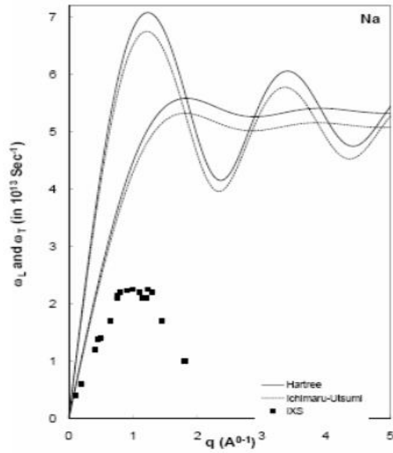
Fig. 2. Phonon dispersion curves of liquid Na.
