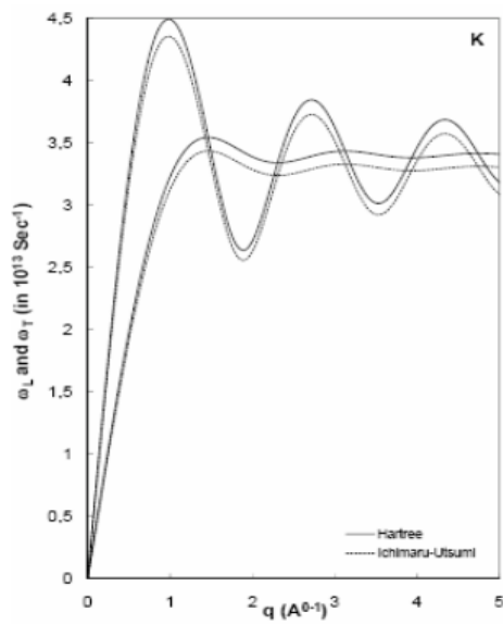
Fig. 3. Phonon dispersion curves of liquid K.
